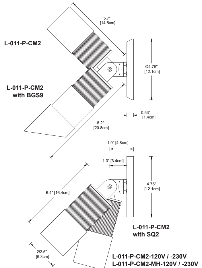
Metal Halide version shown on SQ2 square canopy substitution
